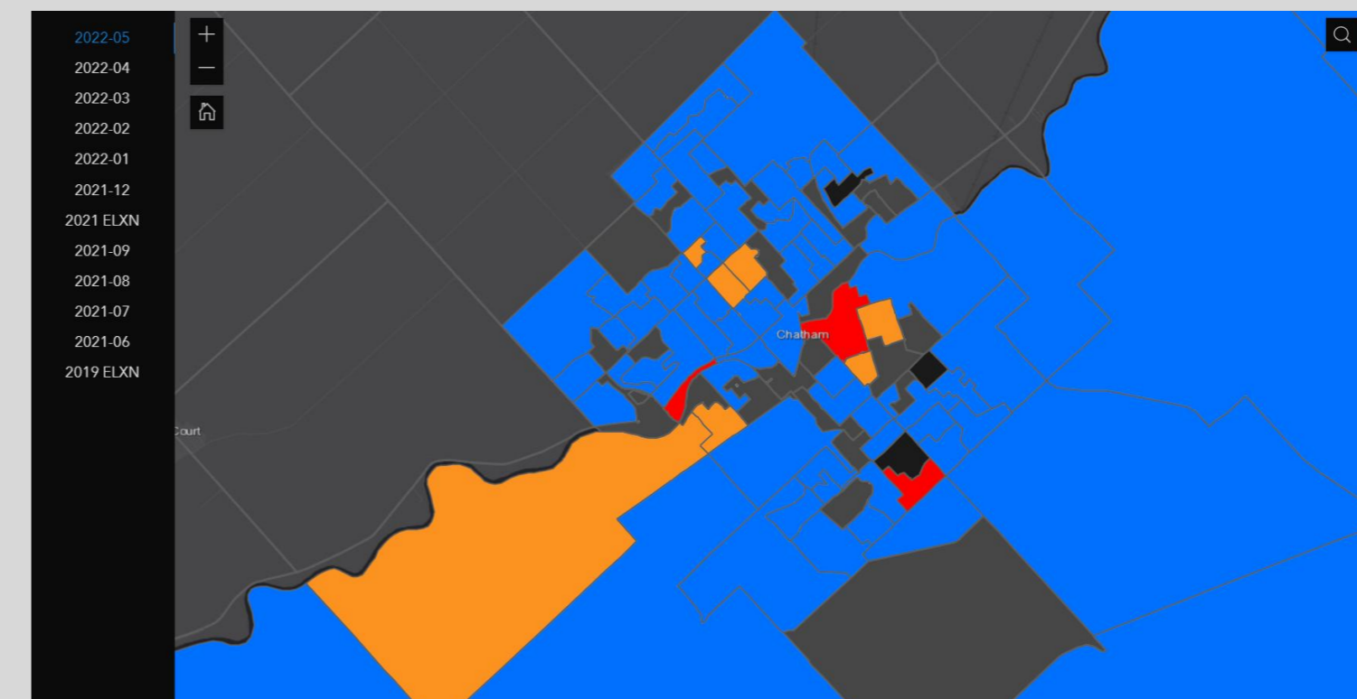
Model Estimate Map Series Trends
